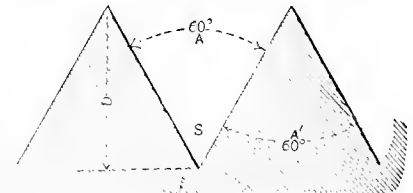
Fig. 5495. V SCREW-THREAD.
